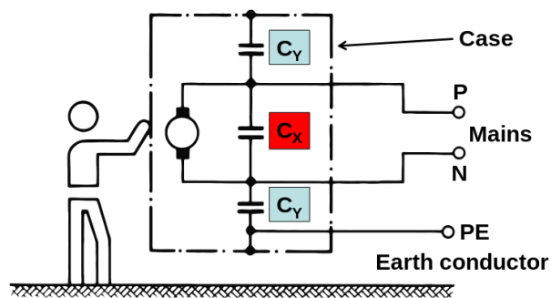
Appliance Class I: Case connected to electrical earth (ground)
